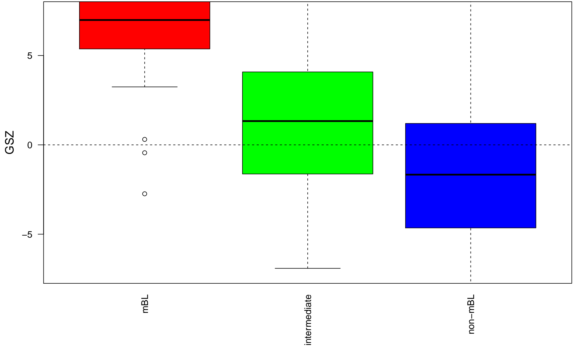
Tirosh_top50 correlated genes PC2
